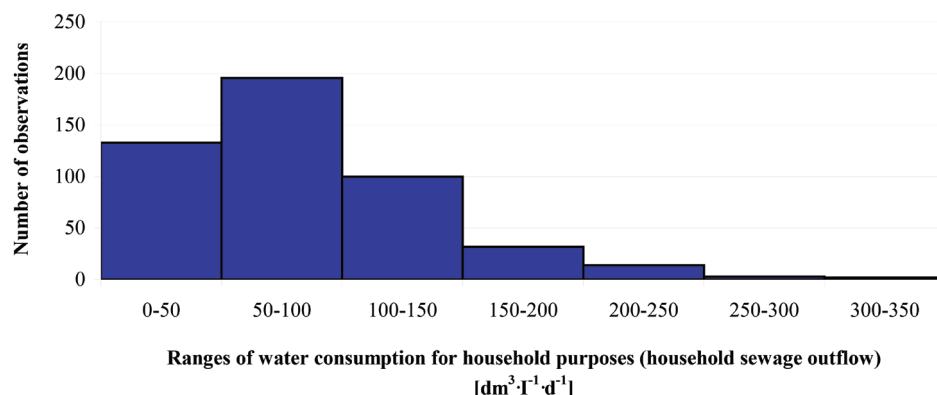
Figure 3. Histogram of water consumption for household purposes (household sewage outflow) in Przęginia Duchowna village in the years 2011-2014
