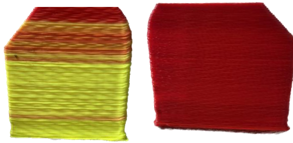
Fig. 7. Printing difference between old cooling (left) and new cooling system (right)
