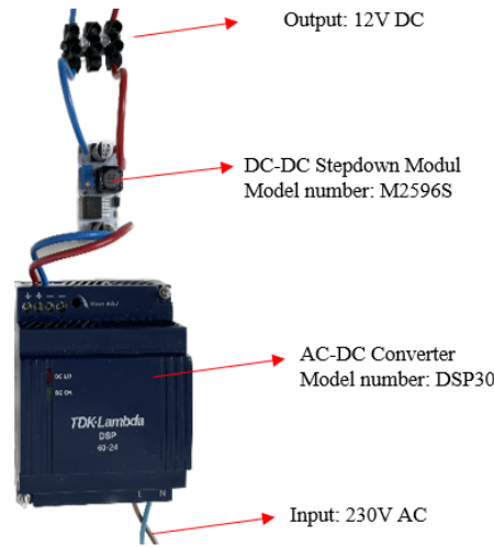
Fig. 5. Electrical construction
