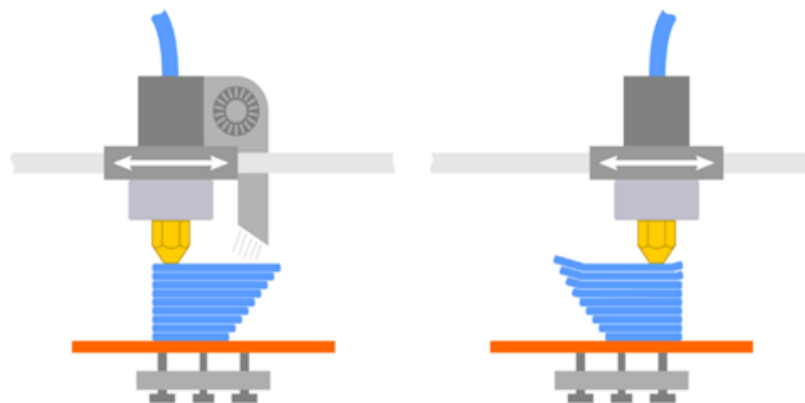
Fig. 2. A printed object with cooling on the left, a printed object without cooling on the right [3]
