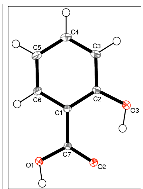
Figure S11. ORTEP view of salicylic acid at 90K with 50% ellipsoid probability (non- H atoms).
