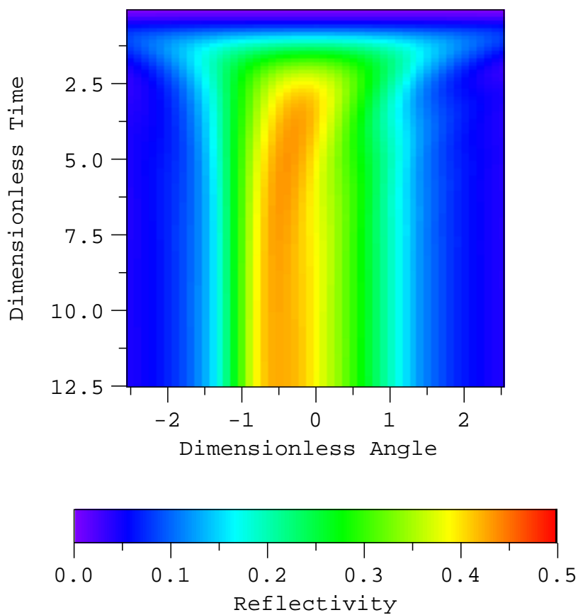
(e) g=-0.5, k=0.25
