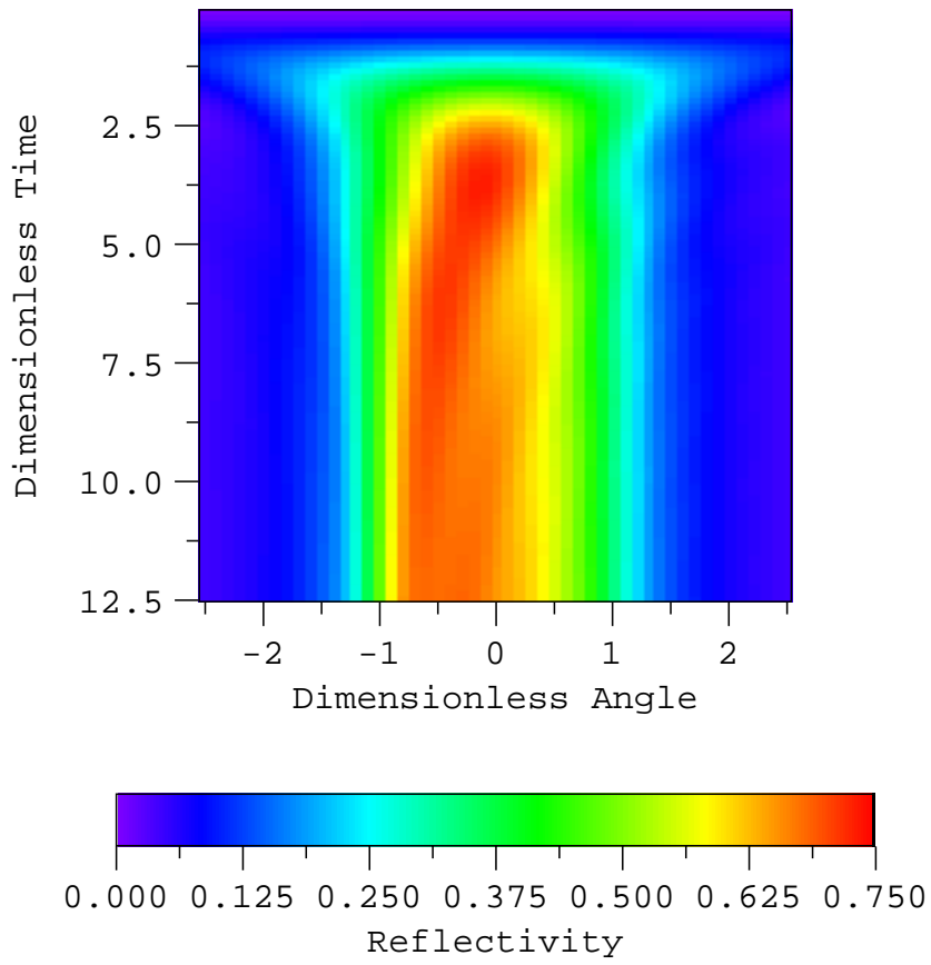
(b) g=-0.2, k=0.1
