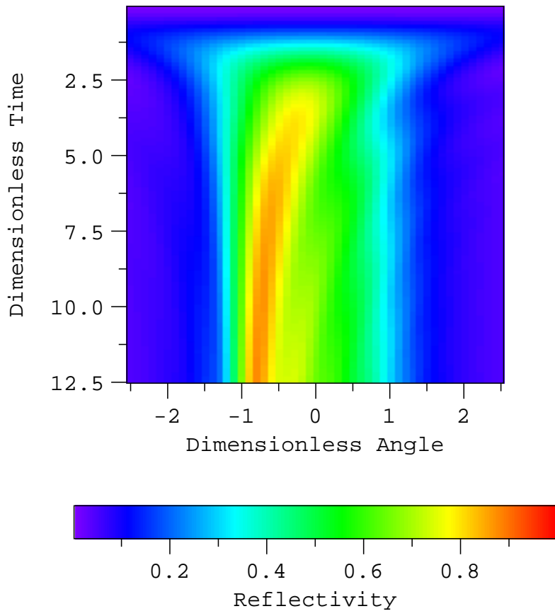
(a) g=-0.2, k=0.199
