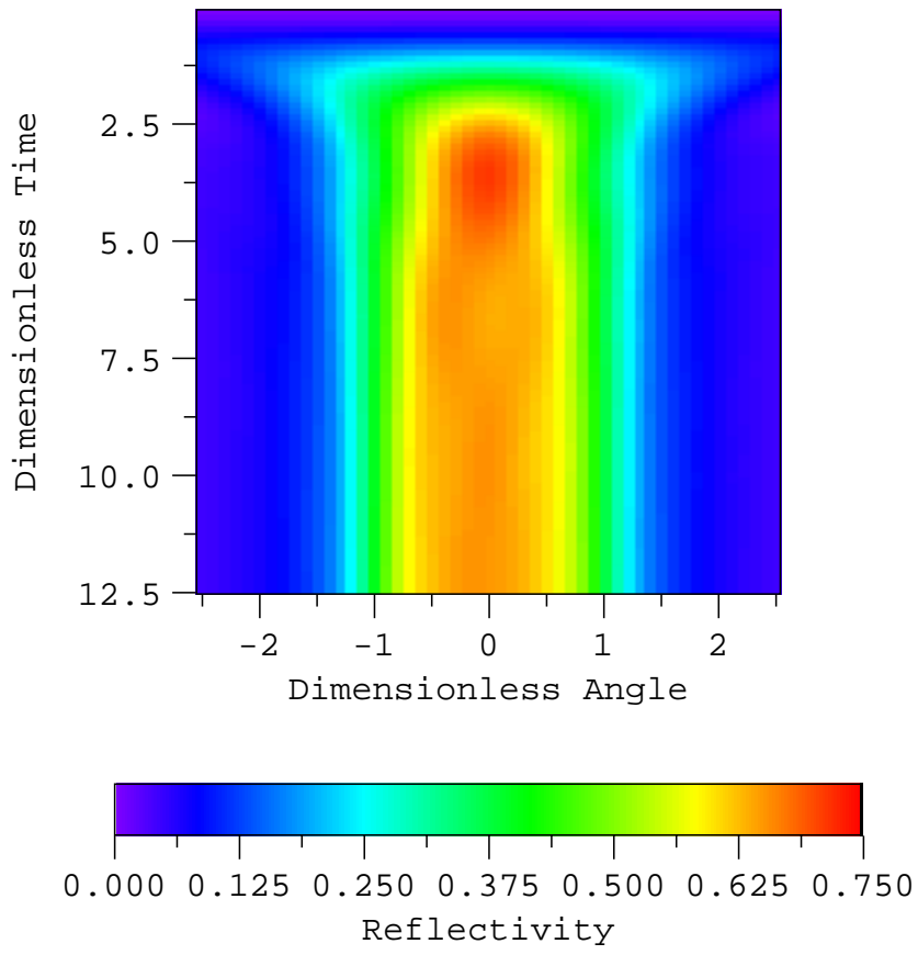
(c) g=-0.2, k=0.02
